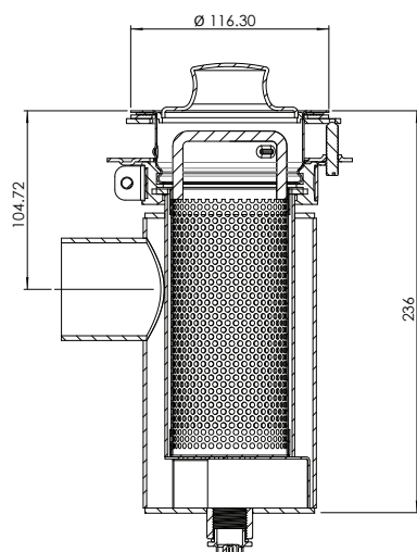
CROSS-SECTION A-A
