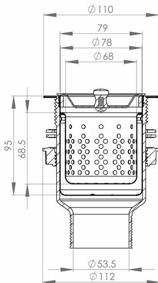
CROSS-SECTION A-A
