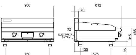
EP516-B
