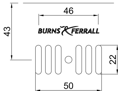
Overflow details A (8:1)
