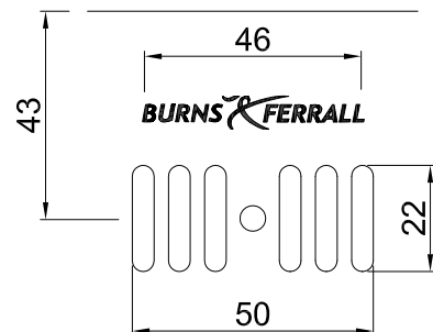
Overflow details A (8:1)
