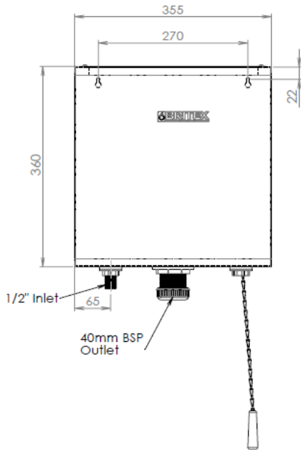
MODEL FCP Front Elevation
