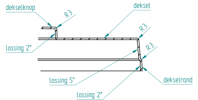
detail B
