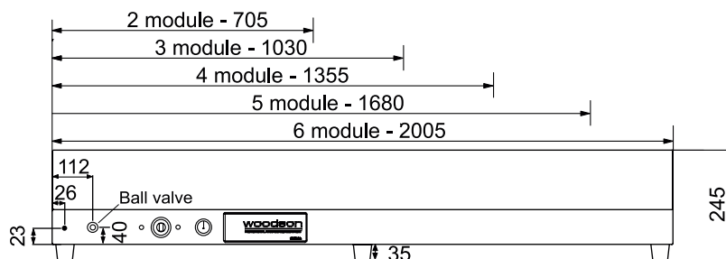
Front View
